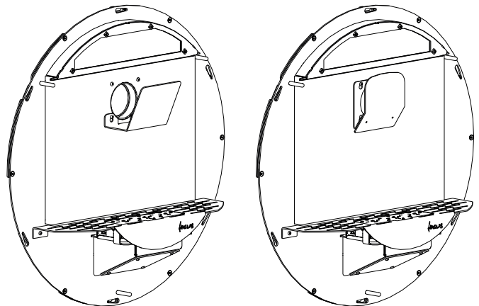
RESTRICTOR A
